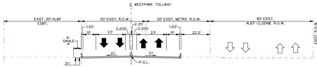
STA. 1112+50 TO STA. 1119+00= STA. 119+00 TO STA. 150+00 (PROPOSED TYPICAL SECTION)
