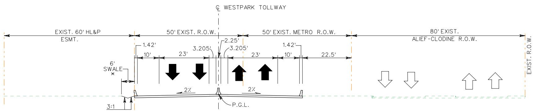
STA. 112+50 TO STA. 1119+00= STA. 119+00 TO STA. 150+00 (PROPOSED TYPICAL SECTION)
